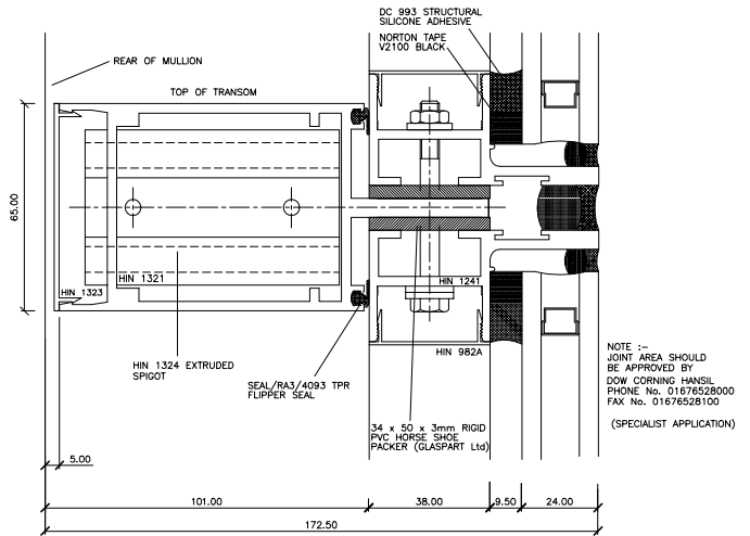
Framed (1241) Transom Detail
