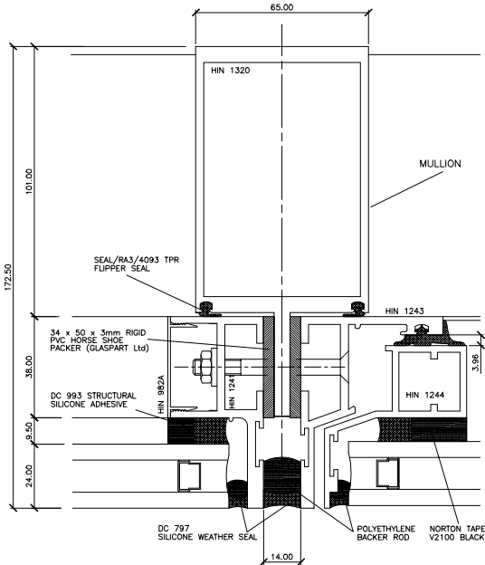
Framed (1241) Mullion Detail With Vent
