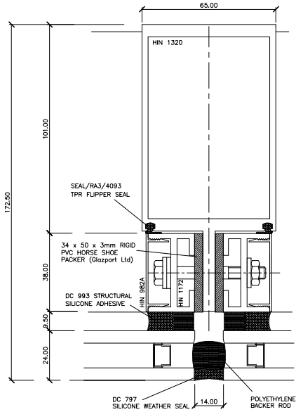
Frameless (1172) Mullion Detail
