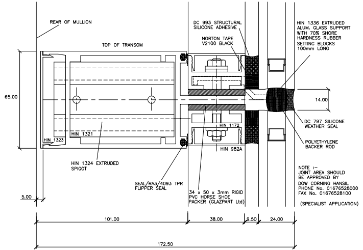
Frameless (1172) Transom Detail
